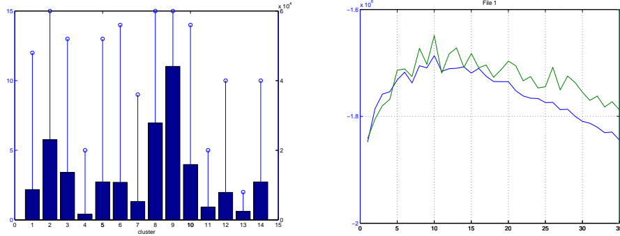
Fig. 1. Thick line (left Y axis): final Gaussian components vs. cluster number; big line (right Y axis): observation number assigned to a cluster vs. cluster number. Fig. 2. Blue line (right Y axis): free energy vs. number of clusters (states); Green line (left Y axis): score K vs. number of clusters; Free energy follows the clustering score.
